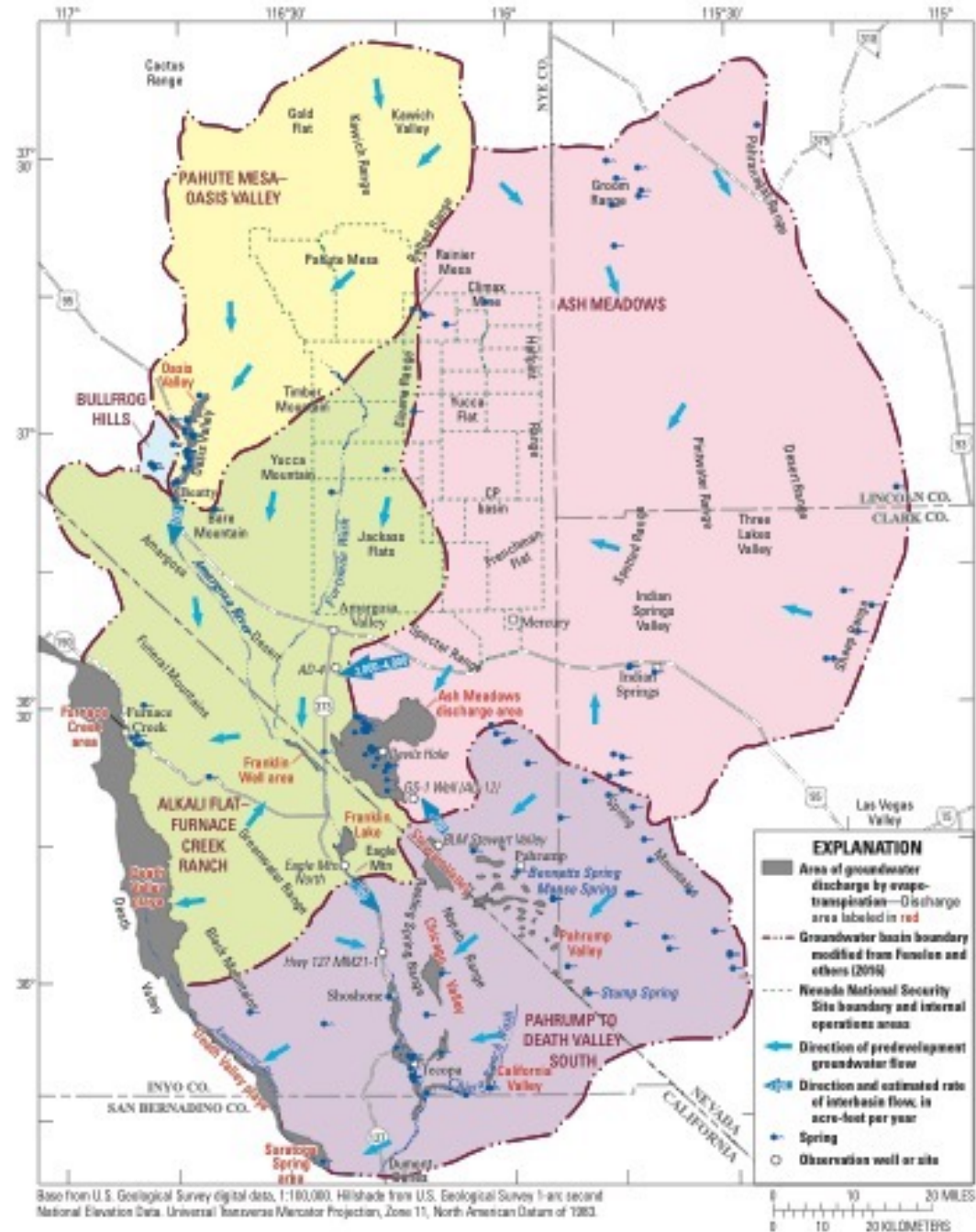
Figure 5. Groundwater basins and major discharge areas in the study area, Nevada and California.
