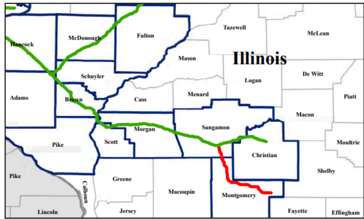
Proposed Illinois portion of Navigator Heartland Greenway CO2 pipeline
